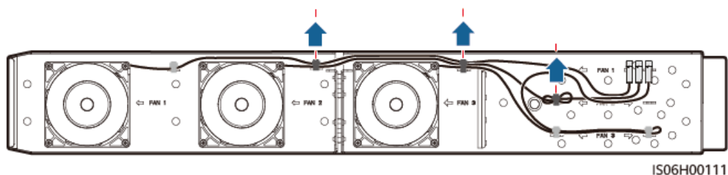
Figura 7-6 Removendo as braçadeiras do FAN 2
