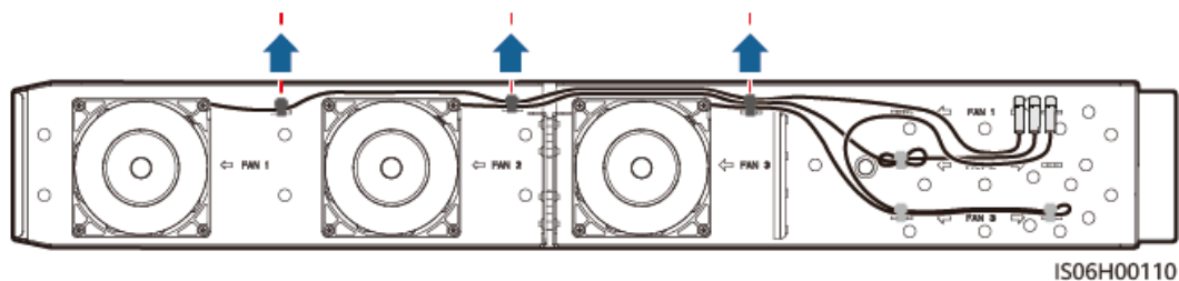
Figura 7-5 Removendo as braçadeiras do FAN 1
