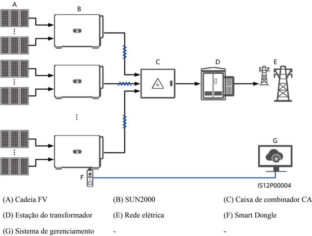
Figura 2-6 Rede do MBUS (Smart Dongle)
