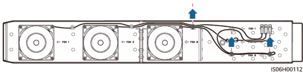
Figura 7-7 Removendo as braçadeiras do FAN 3
