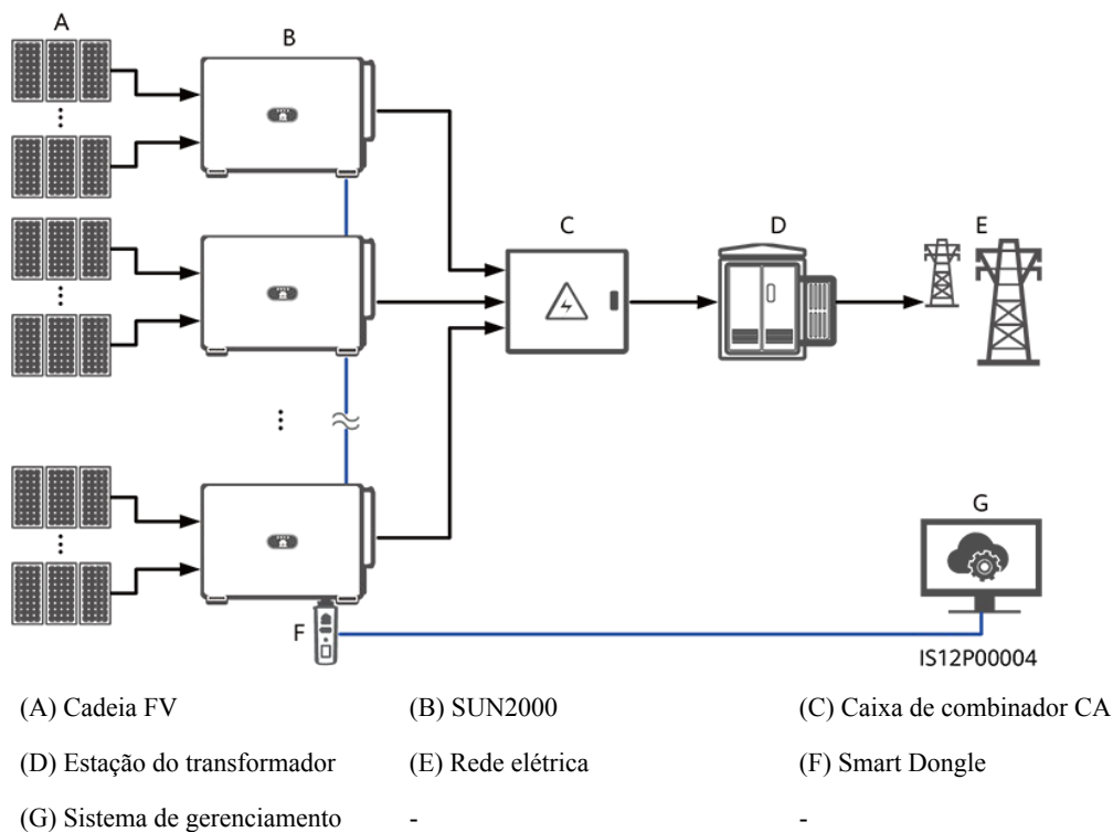
Figura 2-4 Rede RS485 (Smart Dongle)
