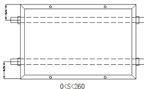
Installation of mounting beam through short side four pressure blocks
