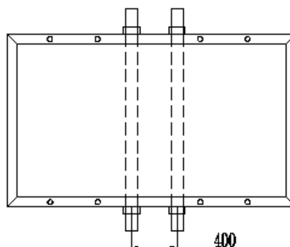
Installation of mounting beam through long side with 400 spacing four pressure blocks
