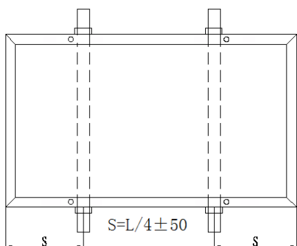
Installation of mounting beam through long side four pressure blocks
